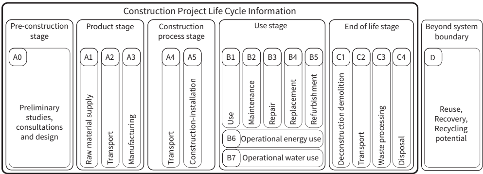
Demand for natural resources and production of waste, greenhouse gases and pollutants occur across the building life cycle (based on EN 15978:2011 and EN 15643-5:2017)
